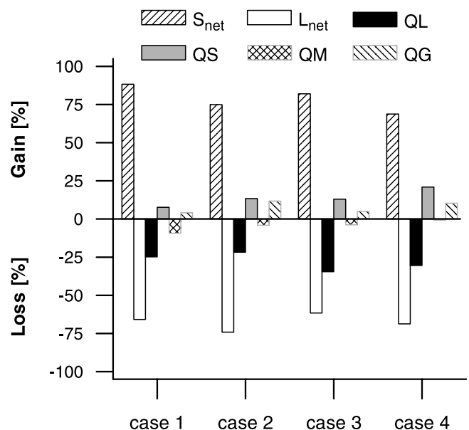
Figure 7. Relative magnitudes of the energy balance components in four different cases (means over the 19 investigated months). Case 1 represents the initial run (Table 2). The energy balance model was also run with offsets in albedo and incoming longwave radiation (case 2) and with increased aerodynamic roughness lengths (case 3), while case 4 combines cases 2 and 3. Details are provided in section 5.
